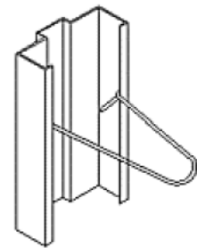
Figure 4B WIRE LOOP ANCHOR (MASONRY)
