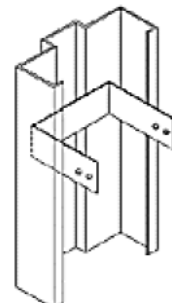
Figure 6B WOOD-STUD ANCHOR
