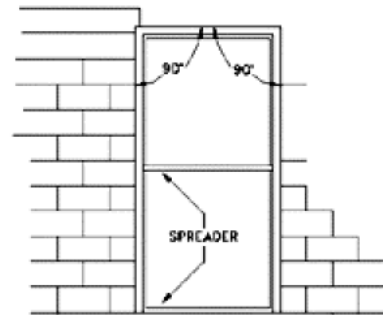
Figure 14 SPREADER LOCATIONS (MASONRY WALLS)
