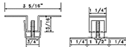
METAL STUD COMPRESSION ANCHORS
