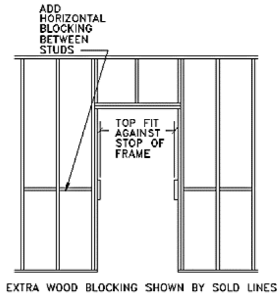
Figure 23 WOOD STUD FRAMING AND BLOCKING FOR KNOCKDOWN FRAME
