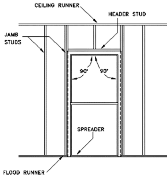
Figure 16 SPREADER LOCATIONS (STEEL STUD WALLS)
