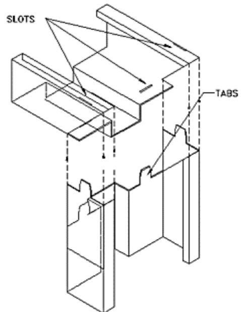
Figure 22 TYPICAL KNOCKDOWN FRAME CORNER CONNECTION
