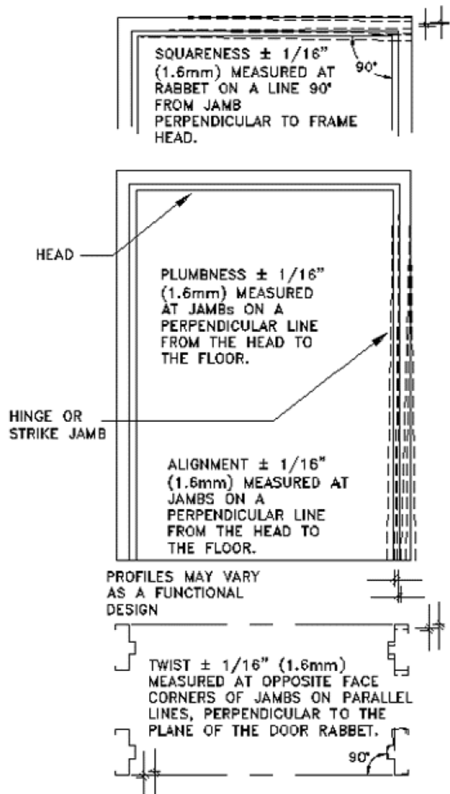
Figure 30 FRAME INSTALLATION TOLERANCES
