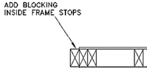
Figure 24 SECTION A-A
