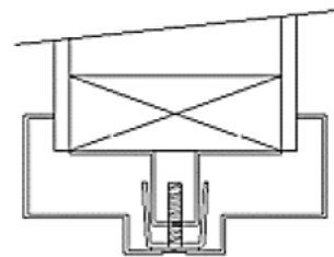
WOOD STUD COMPRESSION ANCHORS
