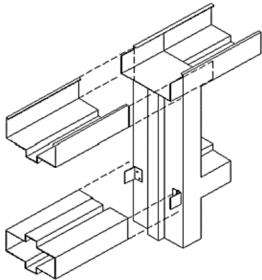
Figure 29 FIELD SPLICES
